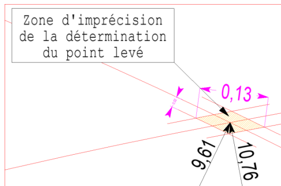
6 Intersection oblique
